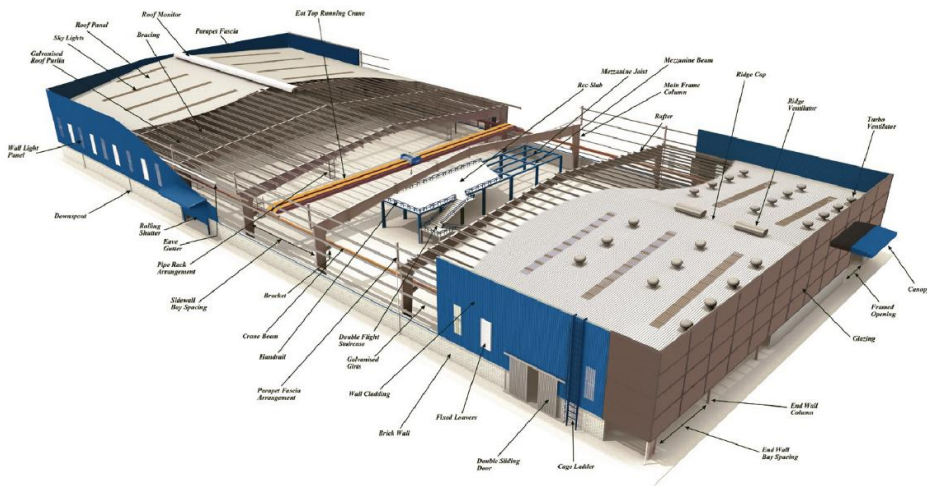
Overall structure of TF steel buliding system
