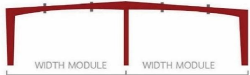
BUILDING WIDTH MAX . PRACTICAL WIDTH = 70 Mtr. MULTI SPAN "1" (TCMS-1)
