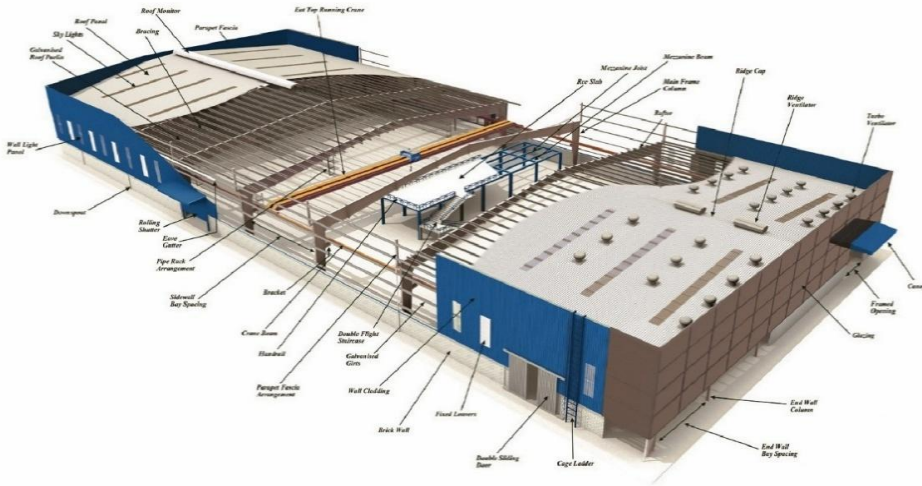
Overall structure of TF steel building system
