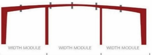
WIDTH MODULE BUILDING WIDTH MAX . PRACTICAL WIDTH = 70 Mtr. MULTI SPAN "2" (TCMS-1)
