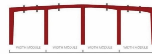
WIDTH MODULE BUILDING WIDTH MAX . PRACTICAL WIDTH = 70 Mtr. MULTI SPAN "3" (TCMS-1)
