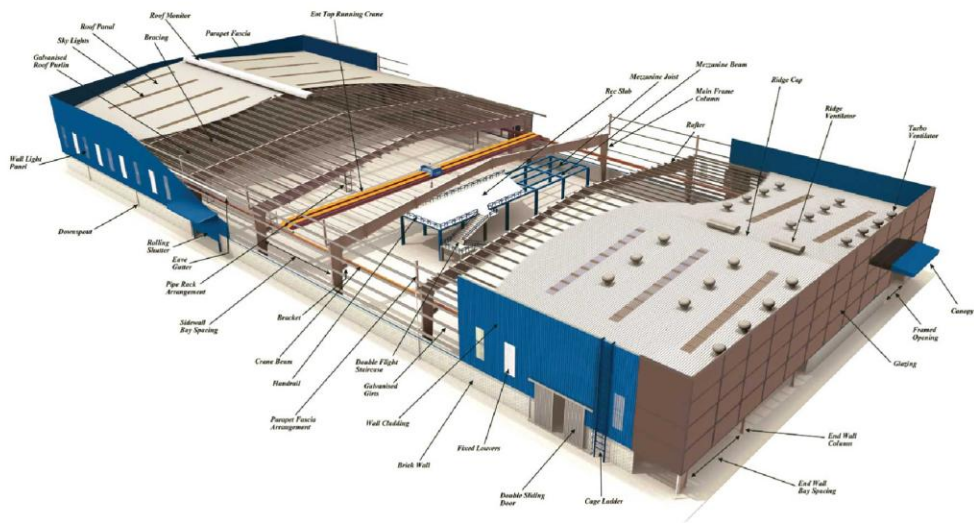
Overall structure of TF steel building system
